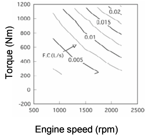
Figure 5.1 Fuel Use Map for a Diesel Engine
